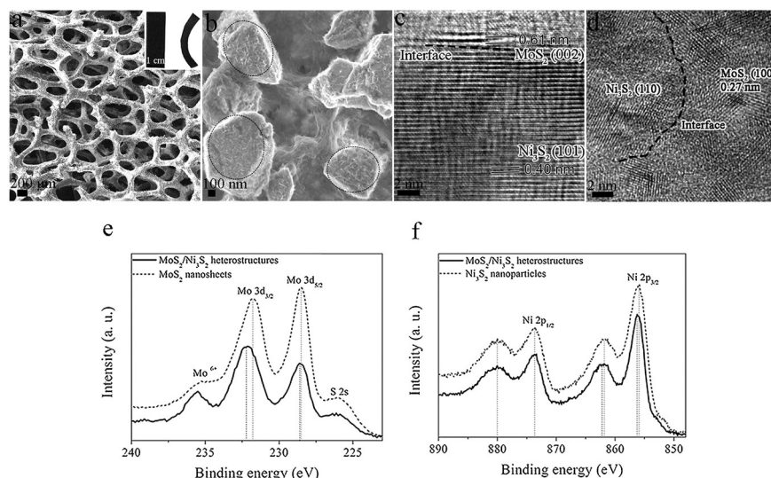
Figure 1. a) and b) scanning electron microscopy and c) and d) high-resolution transmission electron microscopy images of \text{MoS}_2/\text{Ni}_3\text{S}_2 heterostructures. High-resolution X-ray photoelectron spectroscopy spectrum of e) Mo 3d and f) Ni 2p. Inset of (a): digital image of nickel foam coated with \text{MoS}_2/\text{Ni}_3\text{S}_2 heterostructures. The ringed sections of (b) highlight the \text{MoS}_2 nanosheets.
